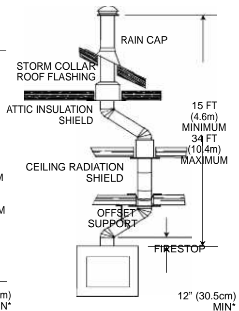
DOUBLE OFF-SET CHIMNEY
